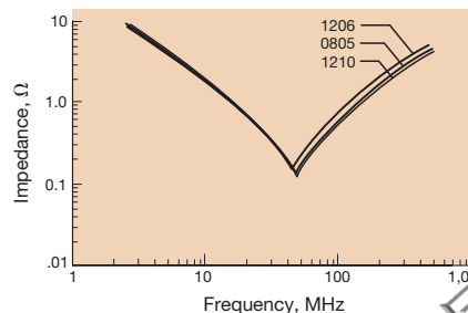
Variation of Impedance with Chip Size Impedance vs. Frequency 10,000 pF - X7S
